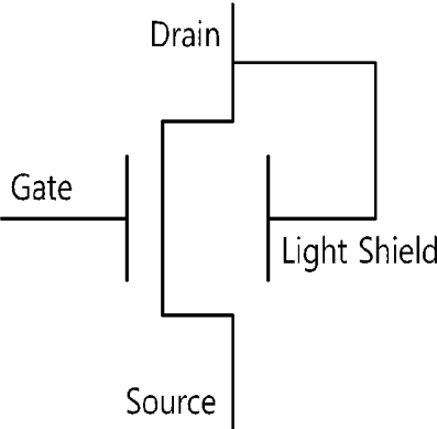
< Drain-LS contact >
